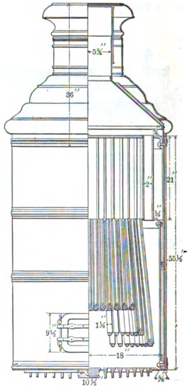
FIG. 44.—FIRE-ENGINE BOILER.
